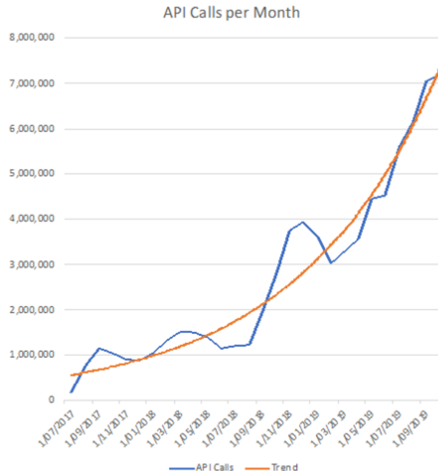
Total calls of community support API on FPT.AI Platform
